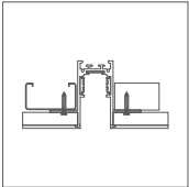
预埋式安装 Pre-embedded type
