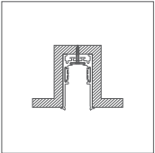
窄边嵌入式安装 Recessed type
