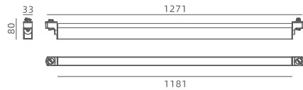
H-LD075-12
