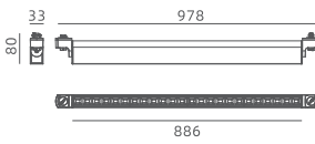
H-LD076-09
