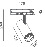
H-LD039MY
