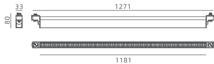
H-LD076-12
